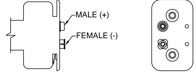
PDSN-20B SNAP TERMINAL
